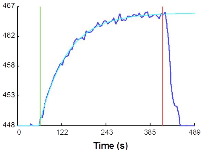
Figure 5: The same accumulation curve as shown in Figure 4, now with appropriate Deadband settings. Note the improved fit (light blue)
