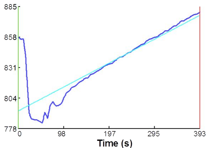
Figure 3. Example of a steady flux of CO 2 , where the initial portion of the accumulation curve has been contaminated by gas from the previous measurement.
