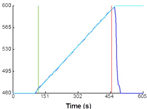
Figure 2. A steady flux of CO 2 suitable for linear fitting. The observed flux (3.99 μmol/m 2 /s) is proportional to the slope of the fitted line.
